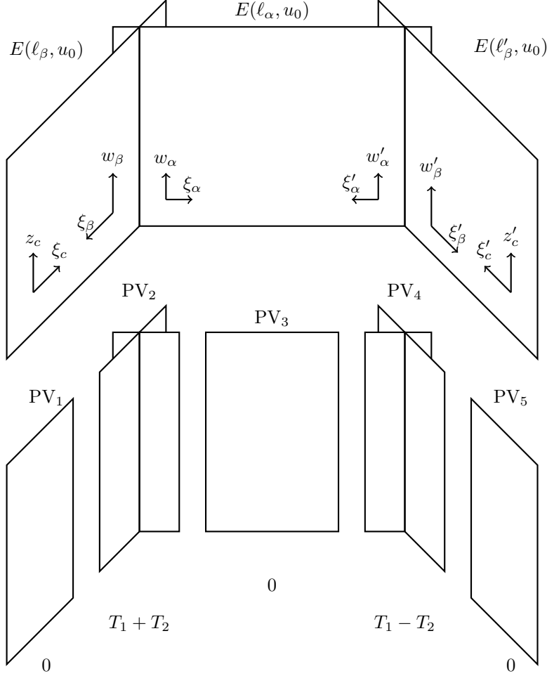
FIGURE 2. This diagram should help to clarify coordinates patches. It also identifies how the principal value integral will be broken into five pieces by truncating the integrals near the poles.
