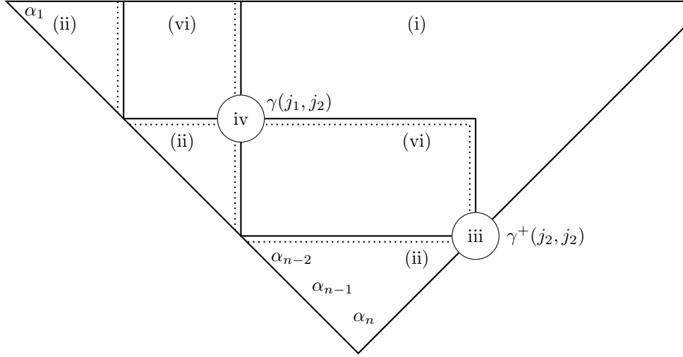
FIGURE 1. This diagram illustrates the p equations for S_1 = \emptyset and |S_2| = 2
